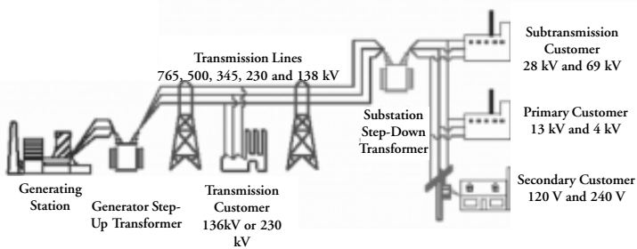
Figure 6. Key Elements of the Electric Power Grid
