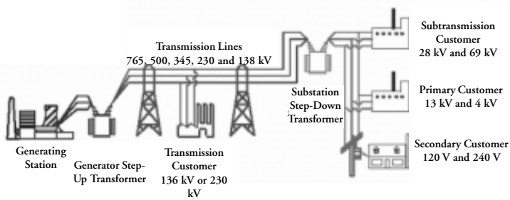
Figure 1. Key Elements of the Electric Power Grid
